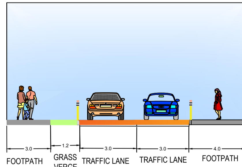
PROPOSED SECTION AT A-A
