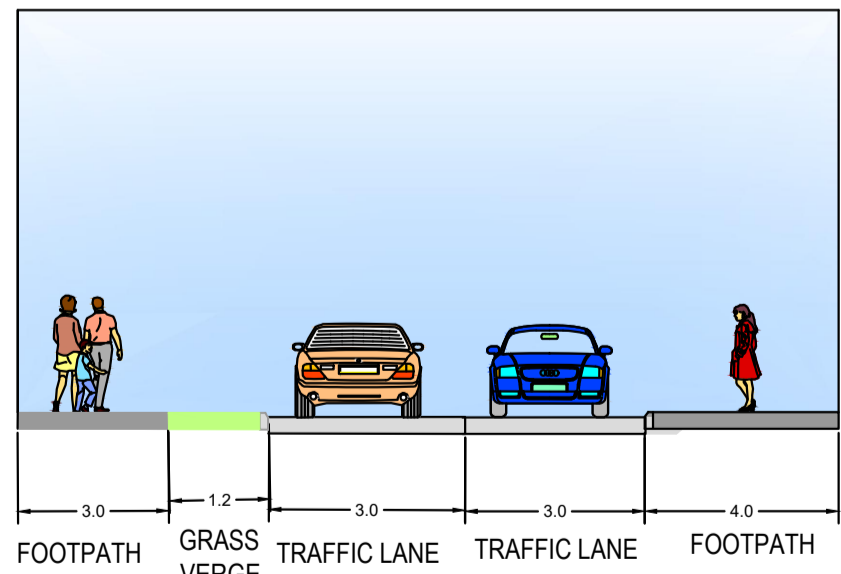
EXISTING CROSS SECTION AT A-A
